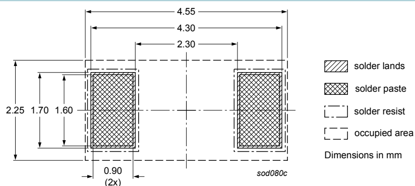
Fig. 7. Reflow soldering footprint for SOD80C (LLDS; MiniMelf)
