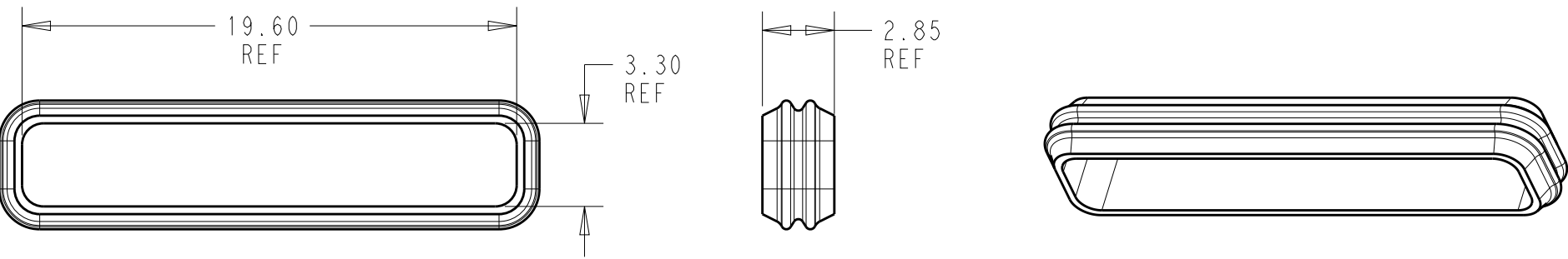
1x8 POSITION
